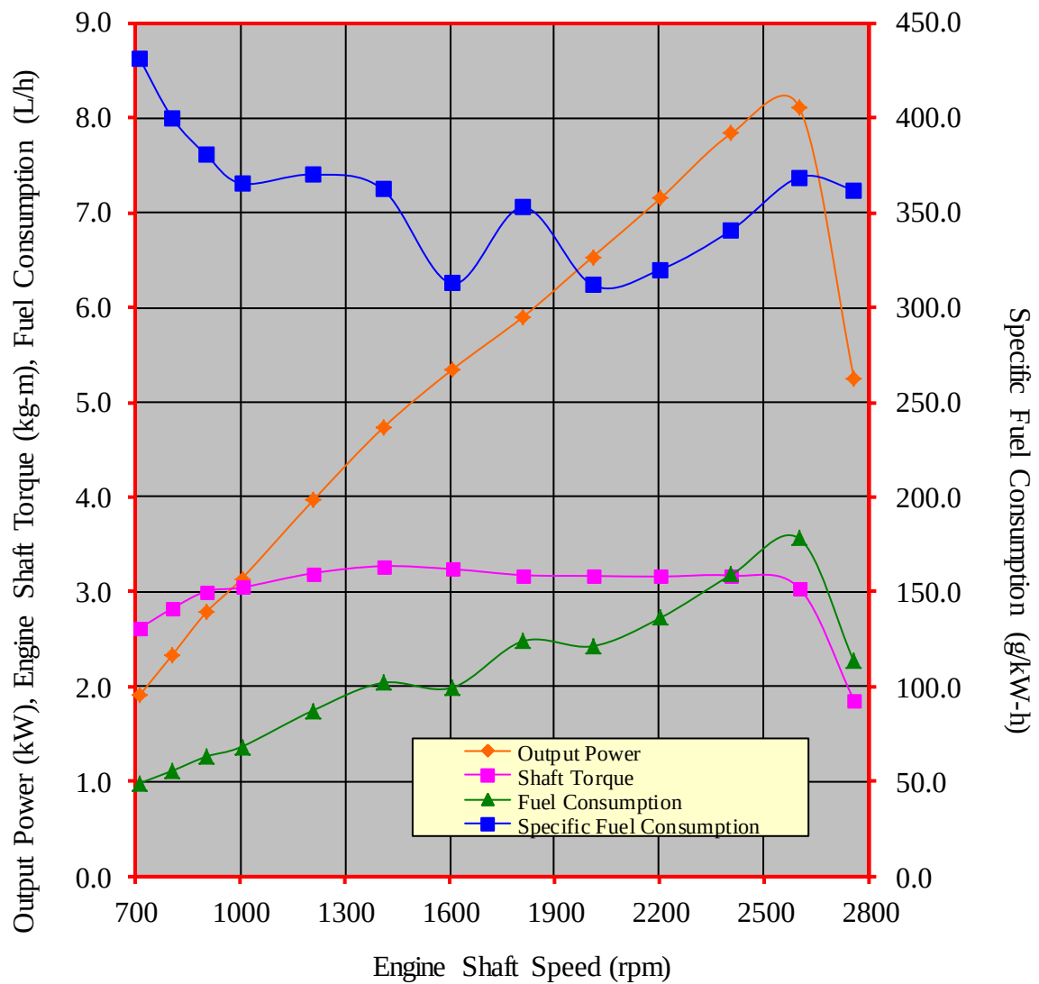
Figure 3. Performance characteristic curves of the MITSUSAN MS110 diesel engine
