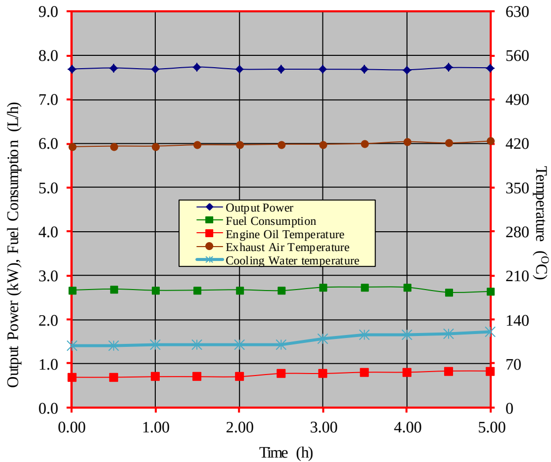
Figure 4. Performance characteristic curves during the continuous running test MITSUSAN MS110 diesel engine
